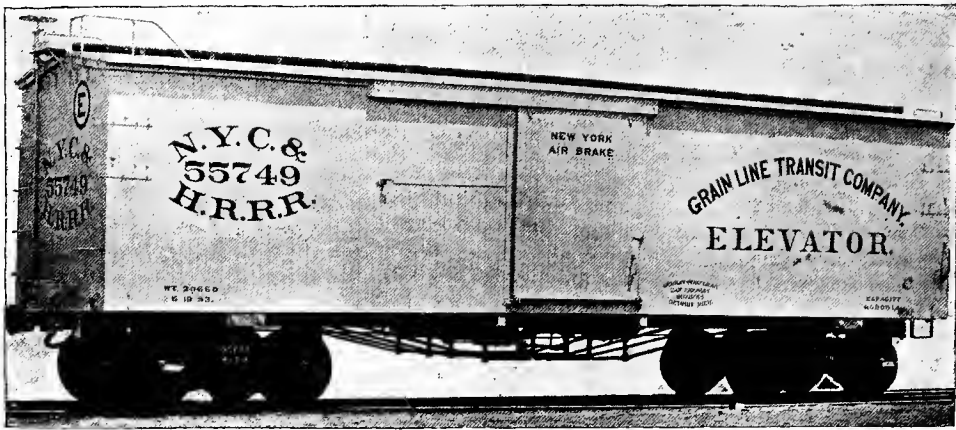
Fig. 1. BOX CAR. NEW YORK CENTRAL & HUDSON RIVER RAILROAD. Capacity, 60,000 lbs. Weight, 30 650 lbs. Inside End Sills, Brake Hand Rail, and Equipped with Air Brakes and For Trucks. (Details are shown in Figs. 227-231.)
